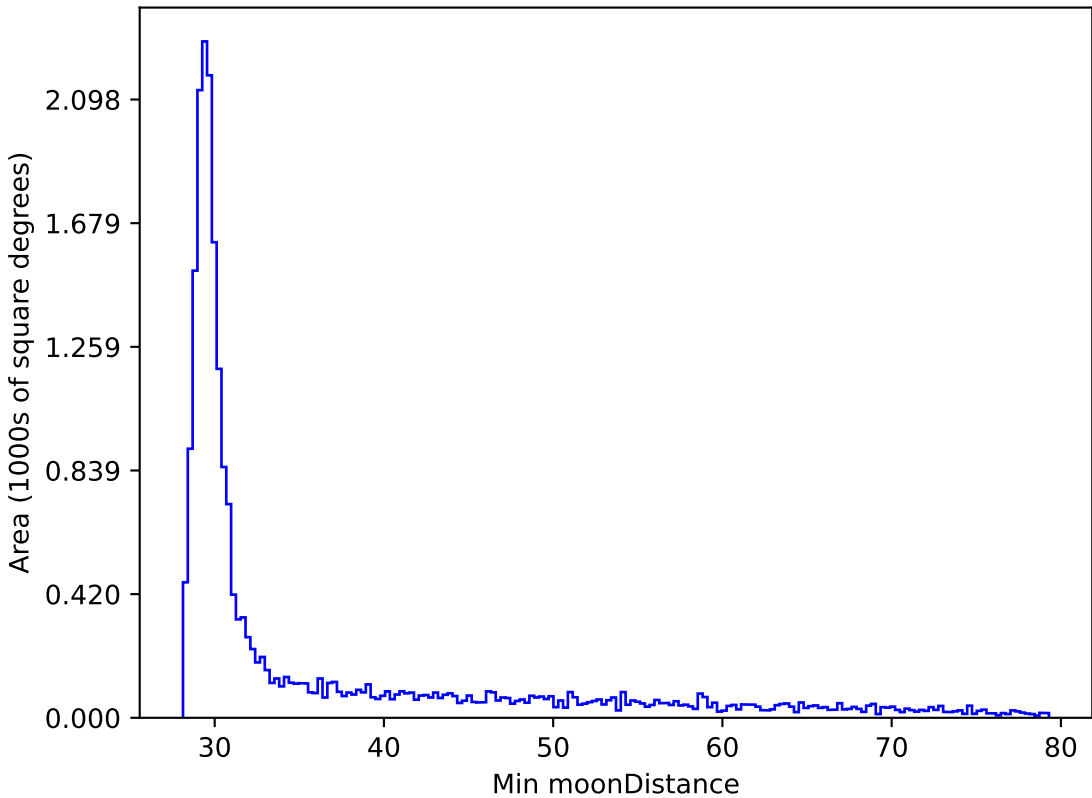
early_u_fpextra4.0_v3.4_10yrs All sky y band: Min moonDistance
