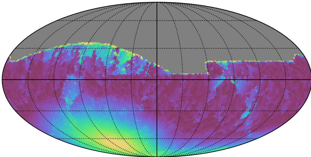
early_u_fpextra4.0_v3.4_10yrs All sky r band: Min moonDistance
