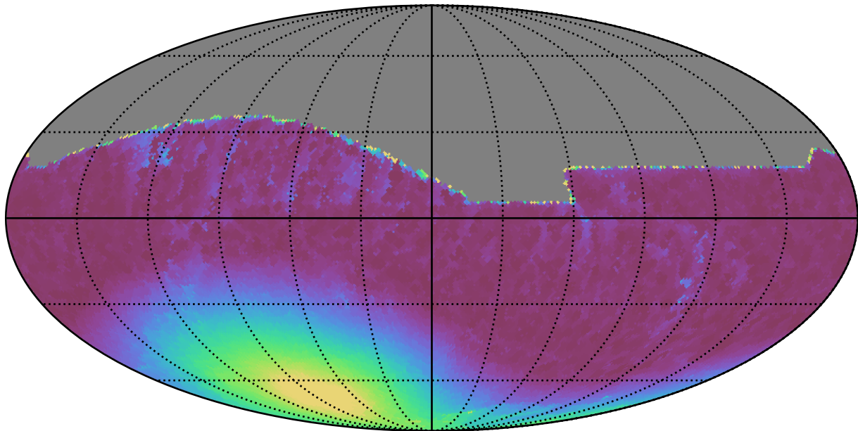
early_u_fpextra4.0_v3.4_10yrs All sky i band: Min moonDistance
