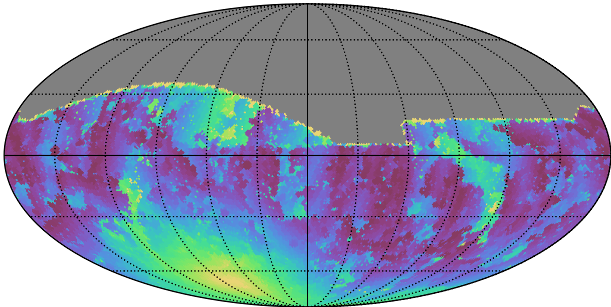
early_u_fpextra4.0_v3.4_10yrs All sky g band: Min moonDistance
