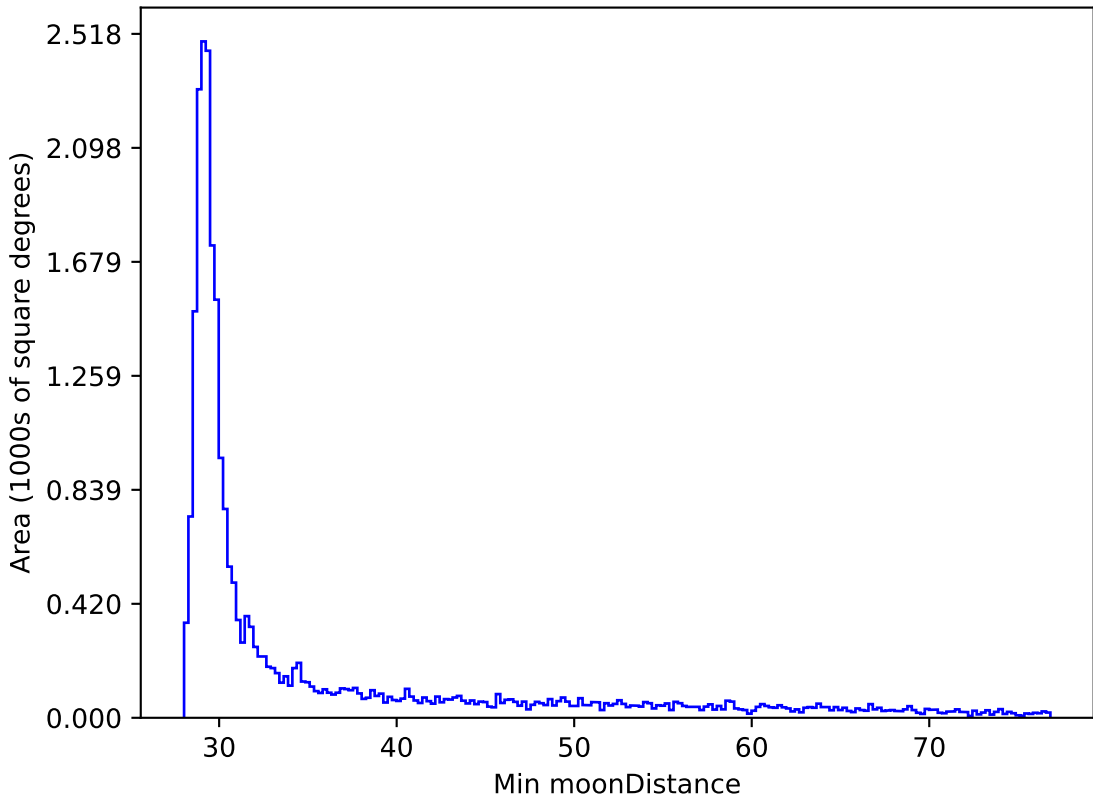
early_u_fpextra4.0_v3.4_10yrs All sky all bands: Min moonDistance
