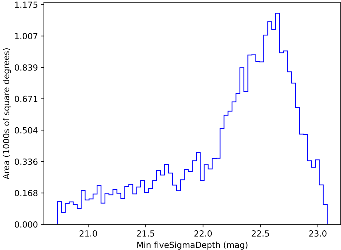
early_u_fpextra4.0_v3.4_10yrs Yr 1 z band: Min fiveSigmaDepth
