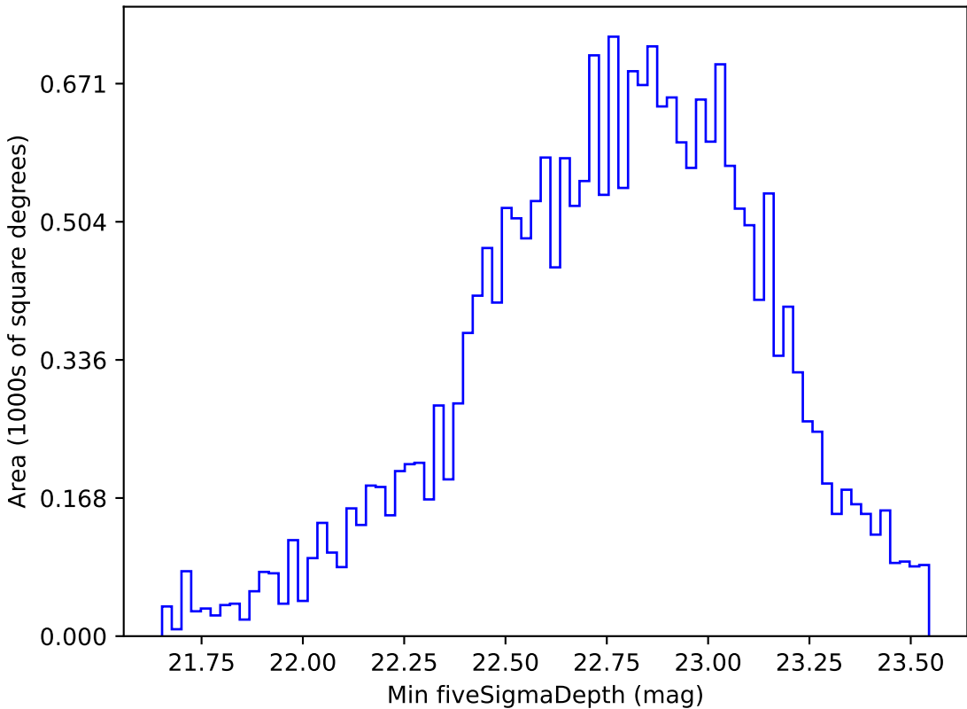
early_u_fpextra4.0_v3.4_10yrs Yr 1 u band: Min fiveSigmaDepth
