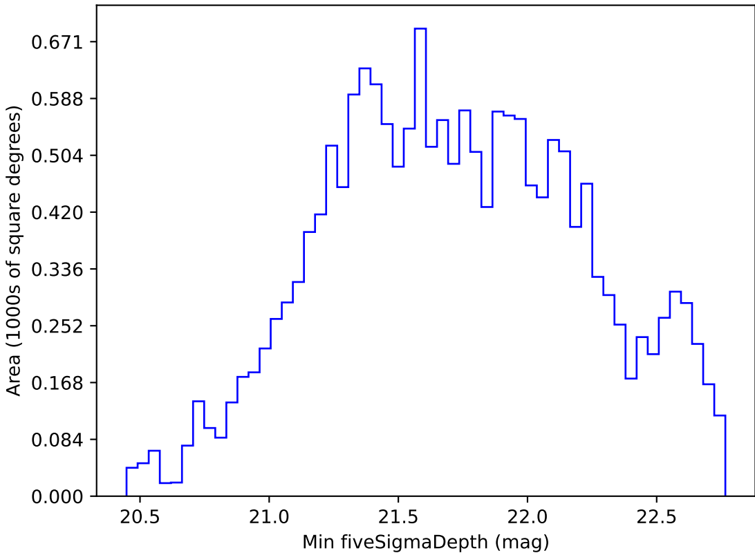
early_u_fpextra4.0_v3.4_10yrs WFD i band: Min fiveSigmaDepth
