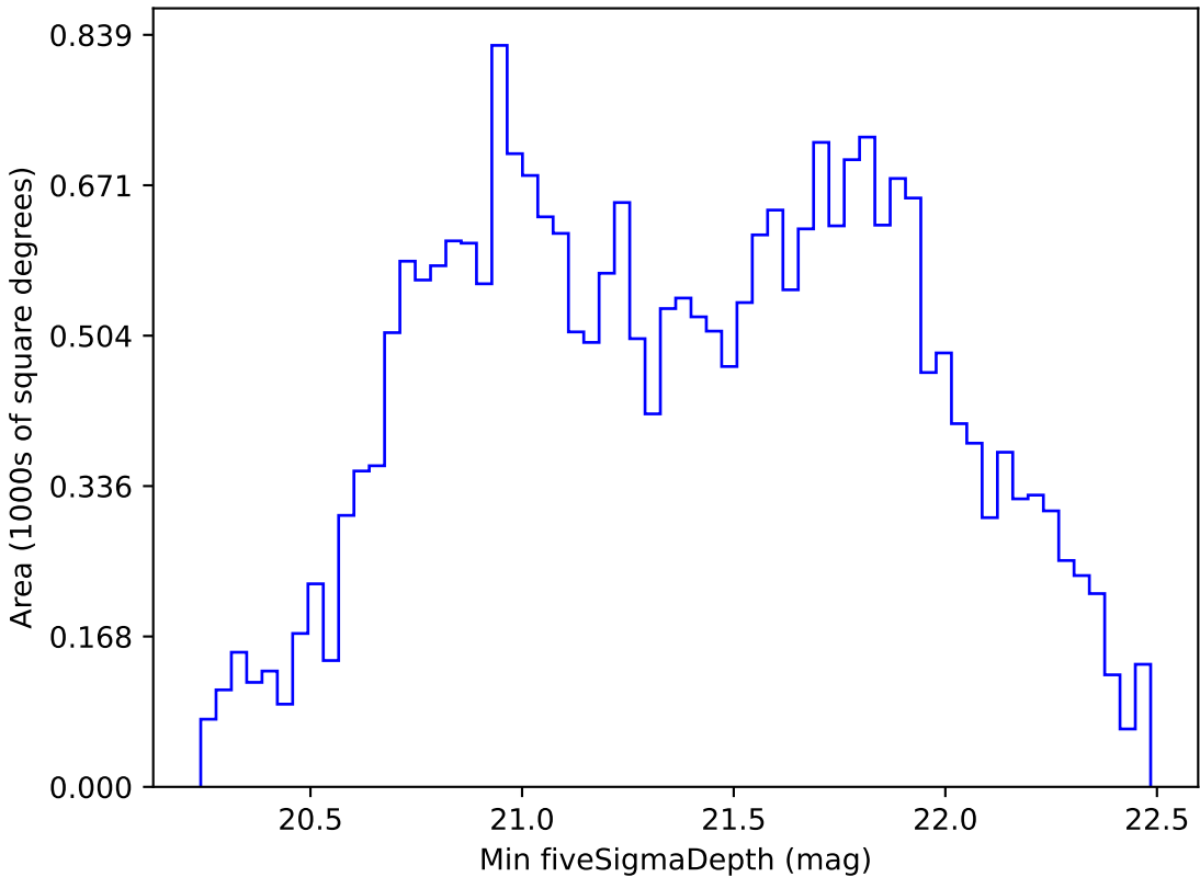
early_u_fpextra4.0_v3.4_10yrs All sky z band: Min fiveSigmaDepth
