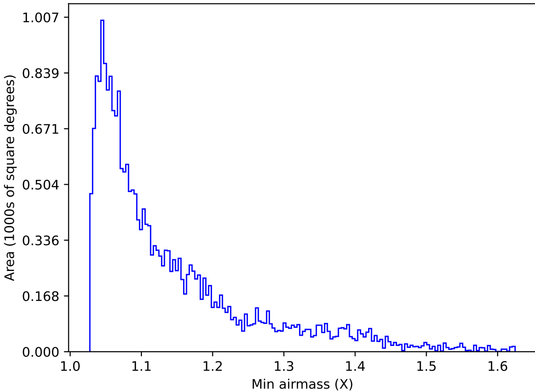
early_u_fpextra4.0_v3.4_10yrs Yr 1 u band: Min airmass
