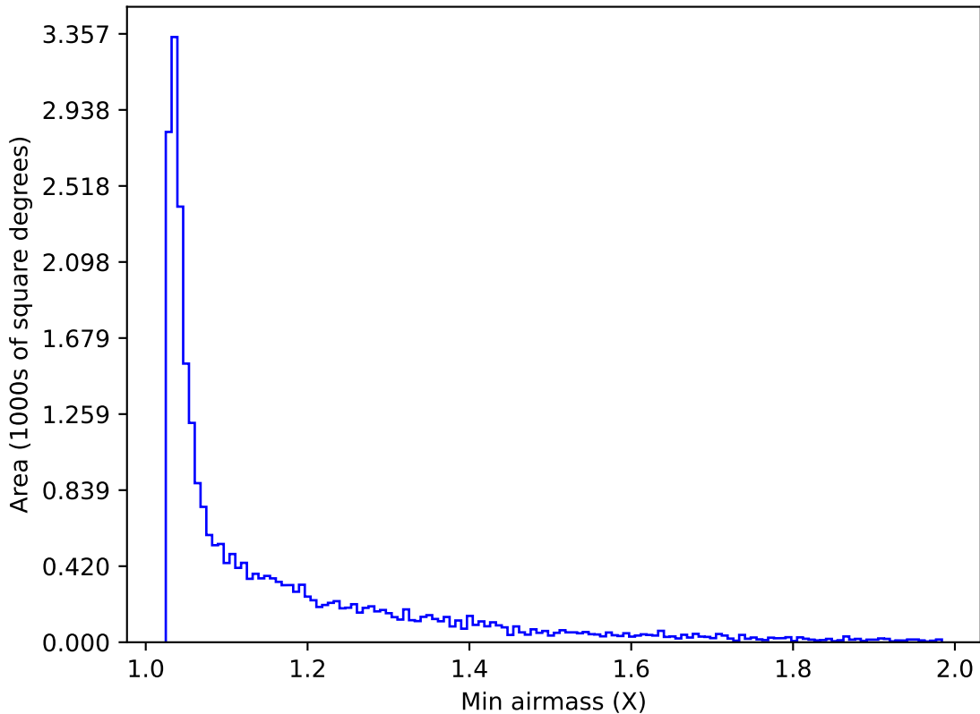
early_u_fpextra4.0_v3.4_10yrs Yr 1 i band: Min airmass
