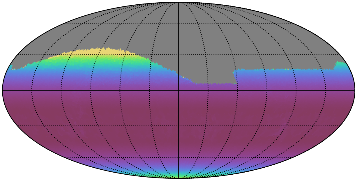
early_u_fpextra4.0_v3.4_10yrs Yr 1 all bands: Min airmass
