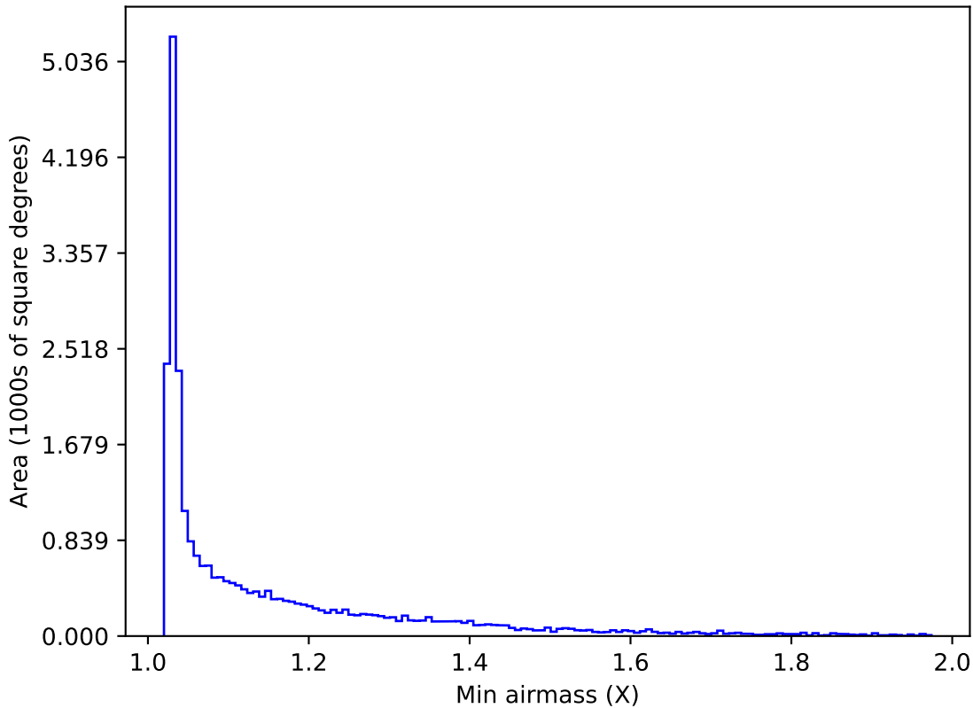
early_u_fpextra4.0_v3.4_10yrs Yr 1 all bands: Min airmass
