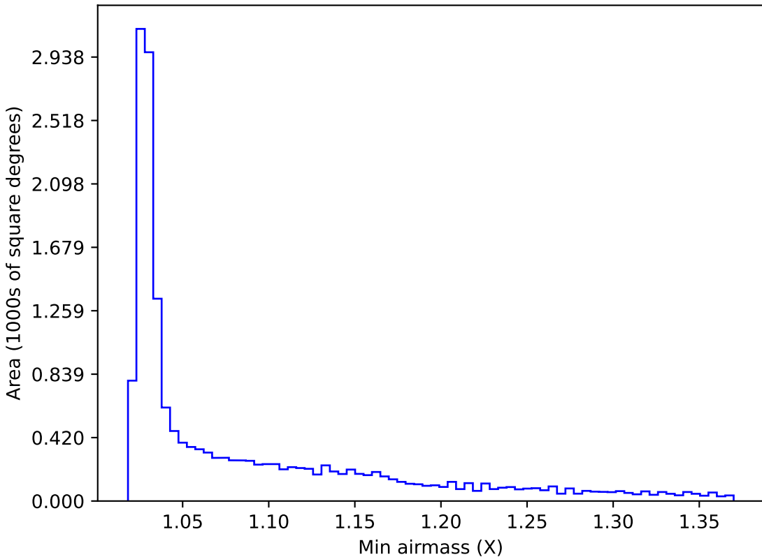
early_u_fpextra4.0_v3.4_10yrs WFD z band: Min airmass
