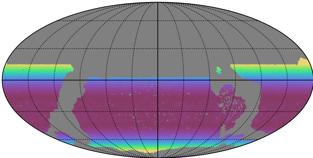
early_u_fpextra4.0_v3.4_10yrs WFD y band: Min airmass
