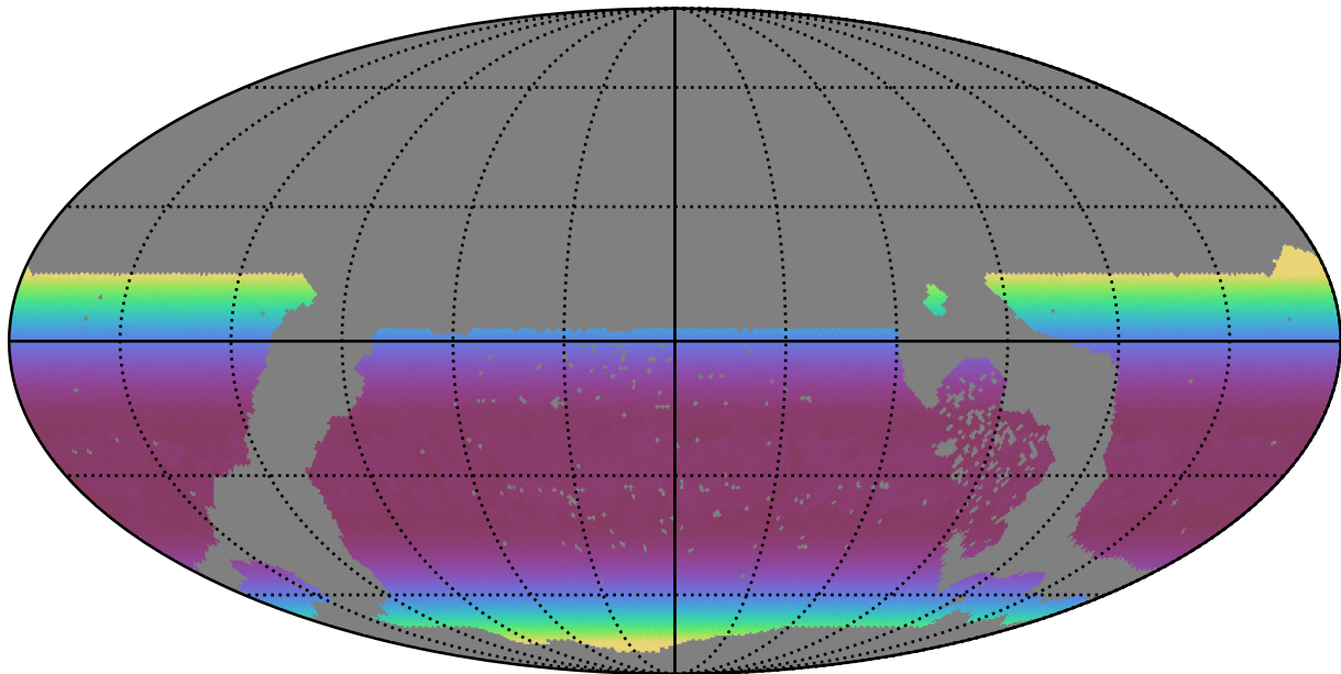
early_u_fpextra4.0_v3.4_10yrs WFD all bands: Min airmass
