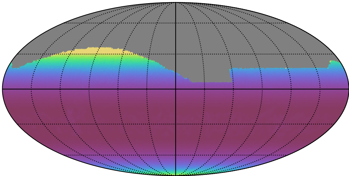
early_u_fpextra4.0_v3.4_10yrs All sky r band: Min airmass
