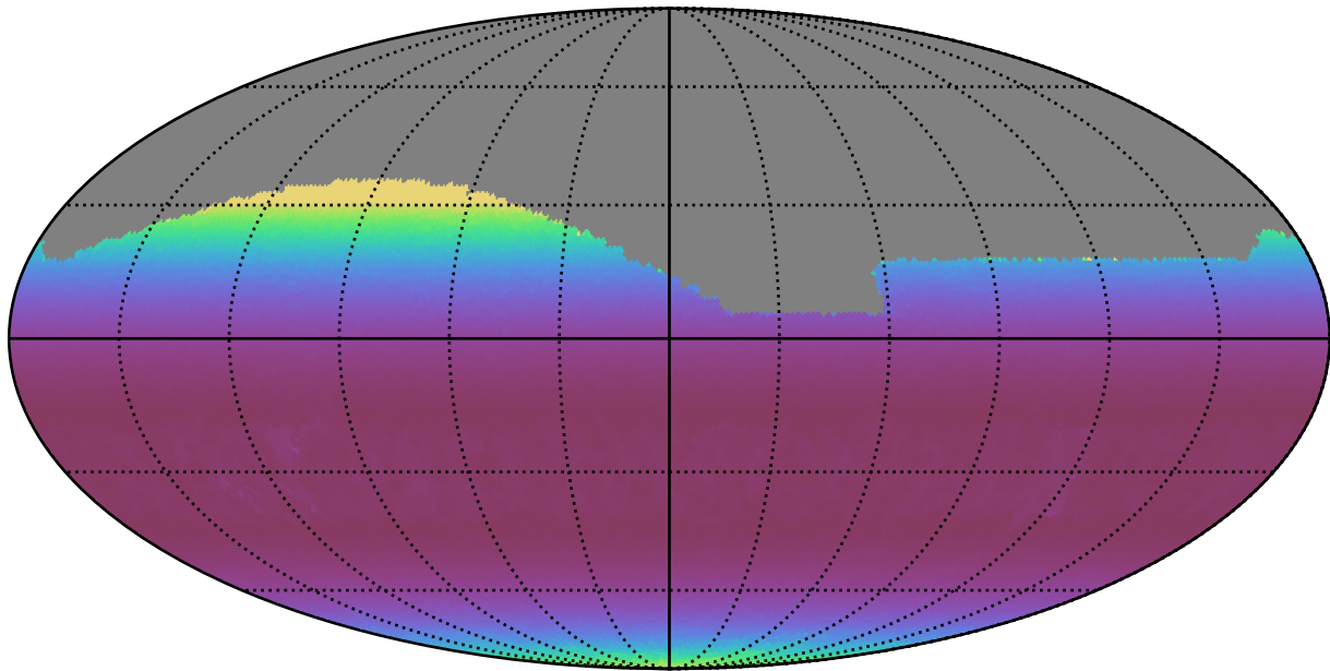
early_u_fpextra4.0_v3.4_10yrs All sky g band: Min airmass
