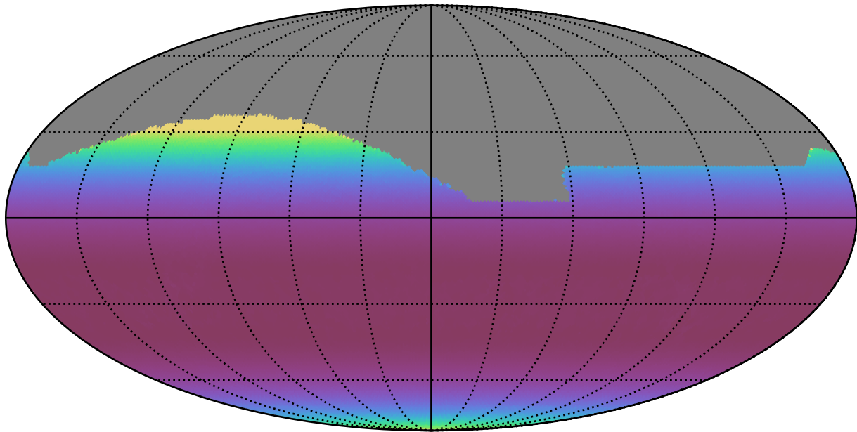
early_u_fpextra4.0_v3.4_10yrs All sky all bands: Min airmass
