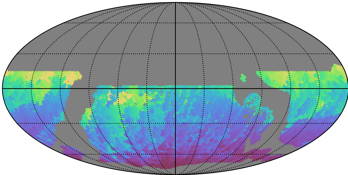
early_u_fpextra4.0_v3.4_10yrs WFD z band: Min HA
