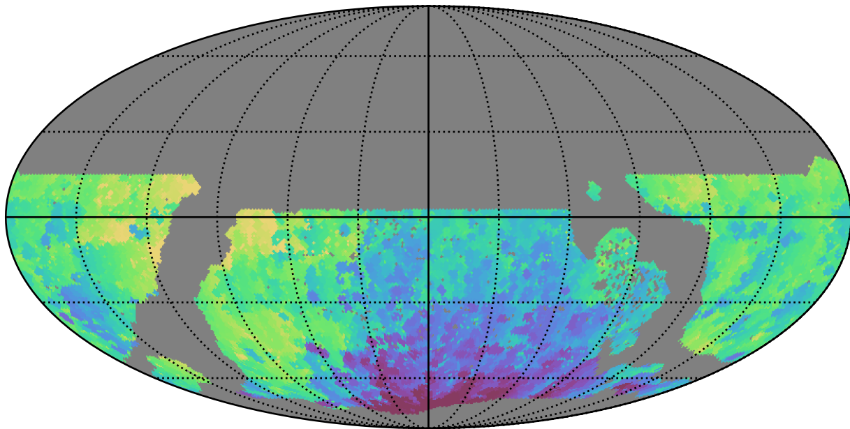
early_u_fpextra4.0_v3.4_10yrs WFD y band: Min HA
