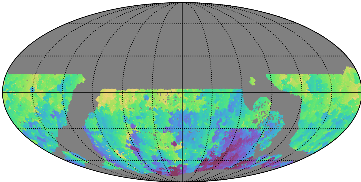
early_u_fpextra4.0_v3.4_10yrs WFD u band: Min HA
