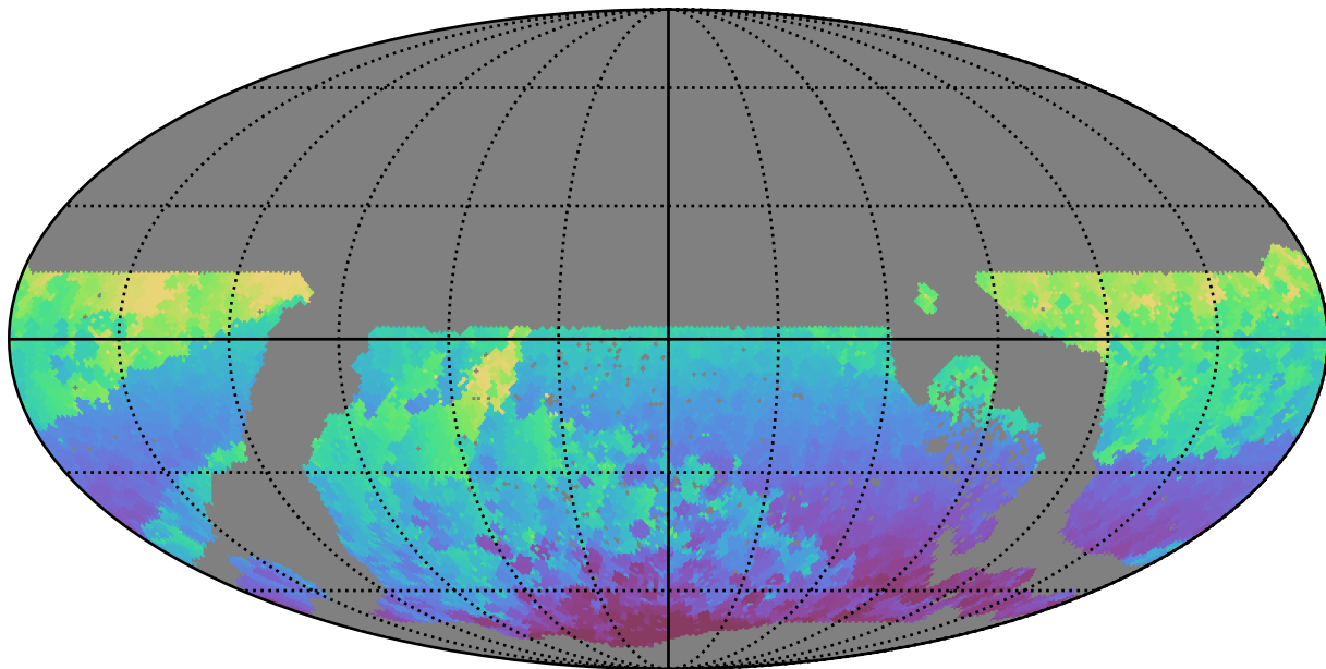
early_u_fpextra4.0_v3.4_10yrs WFD r band: Min HA
