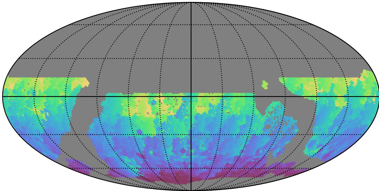
early_u_fpextra4.0_v3.4_10yrs WFD g band: Min HA
