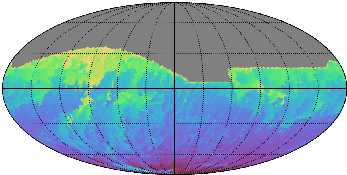
early_u_fpextra4.0_v3.4_10yrs All sky z band: Min HA
