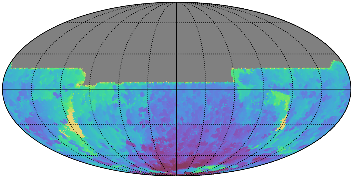
early_u_fpextra4.0_v3.4_10yrs All sky y band: Min HA
