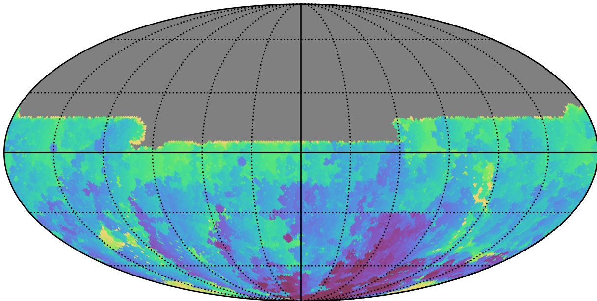
early_u_fpextra4.0_v3.4_10yrs All sky u band: Min HA
