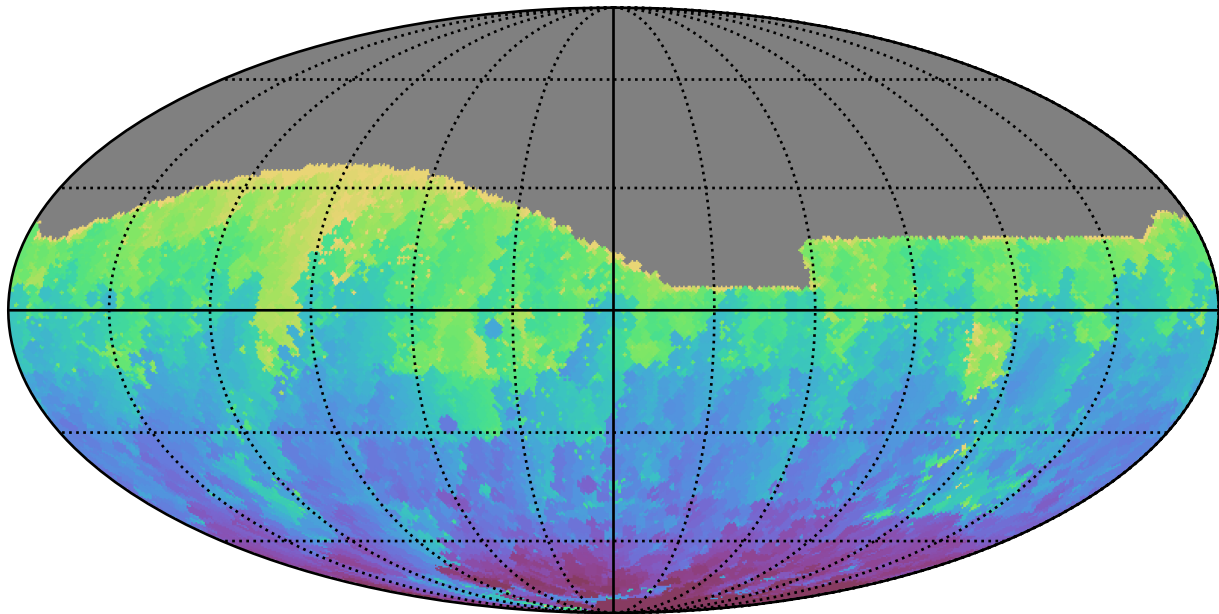
early_u_fpextra4.0_v3.4_10yrs All sky g band: Min HA
