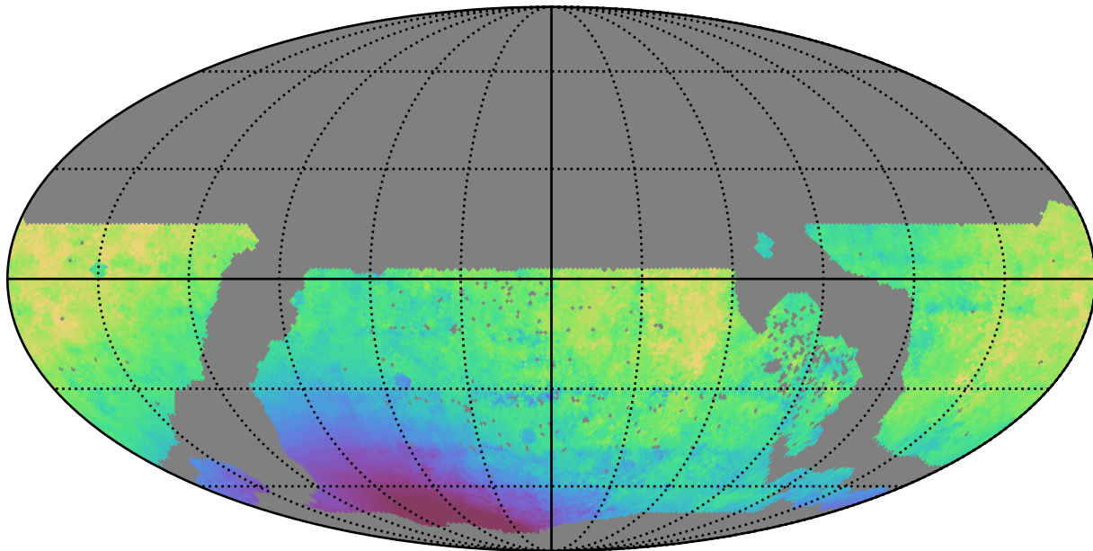
early_u_fpextra4.0_v3.4_10yrs WFD z band: Median solarElong
