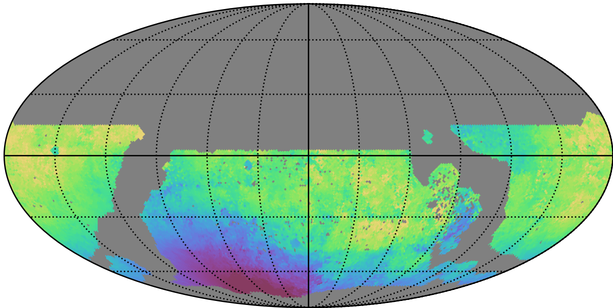
early_u_fpextra4.0_v3.4_10yrs WFD u band: Median solarElong
