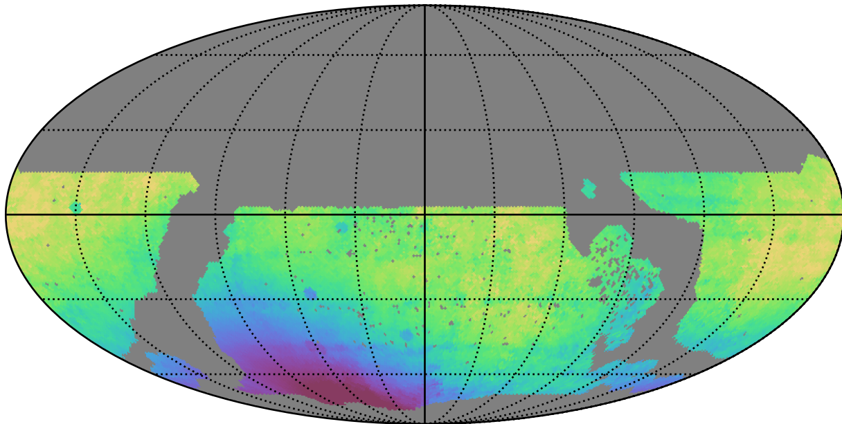
early_u_fpextra4.0_v3.4_10yrs WFD r band: Median solarElong
