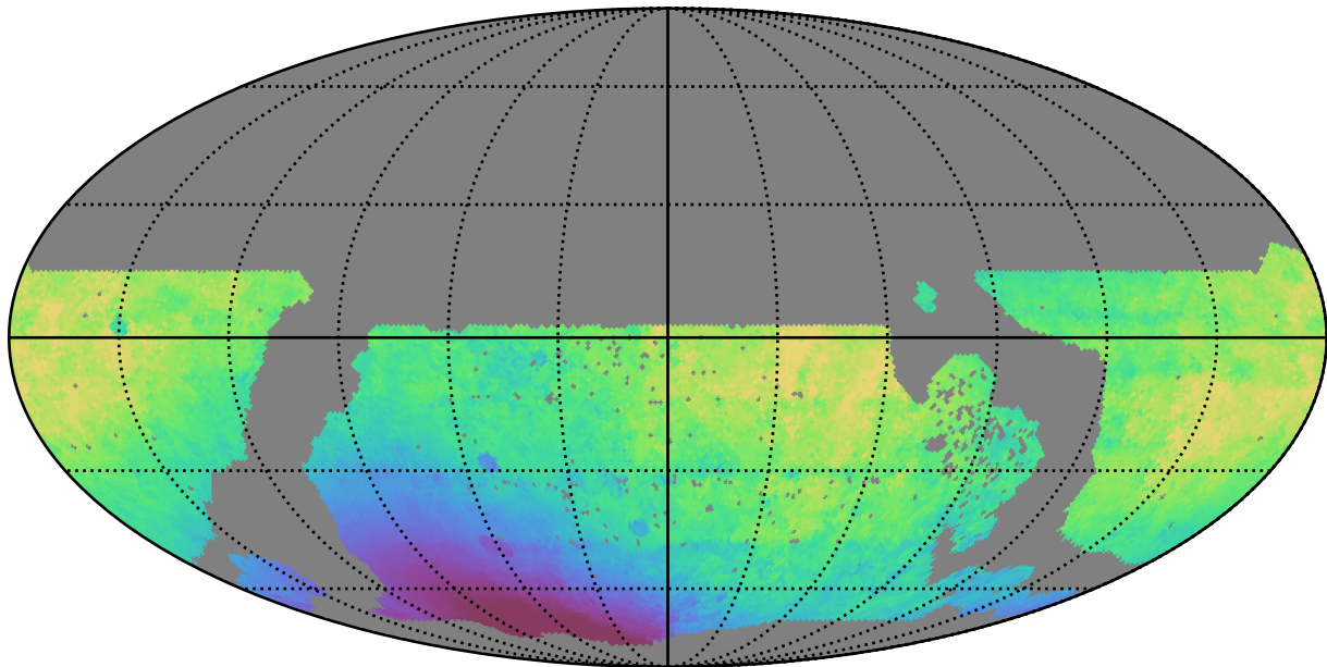
early_u_fpextra4.0_v3.4_10yrs WFD i band: Median solarElong
