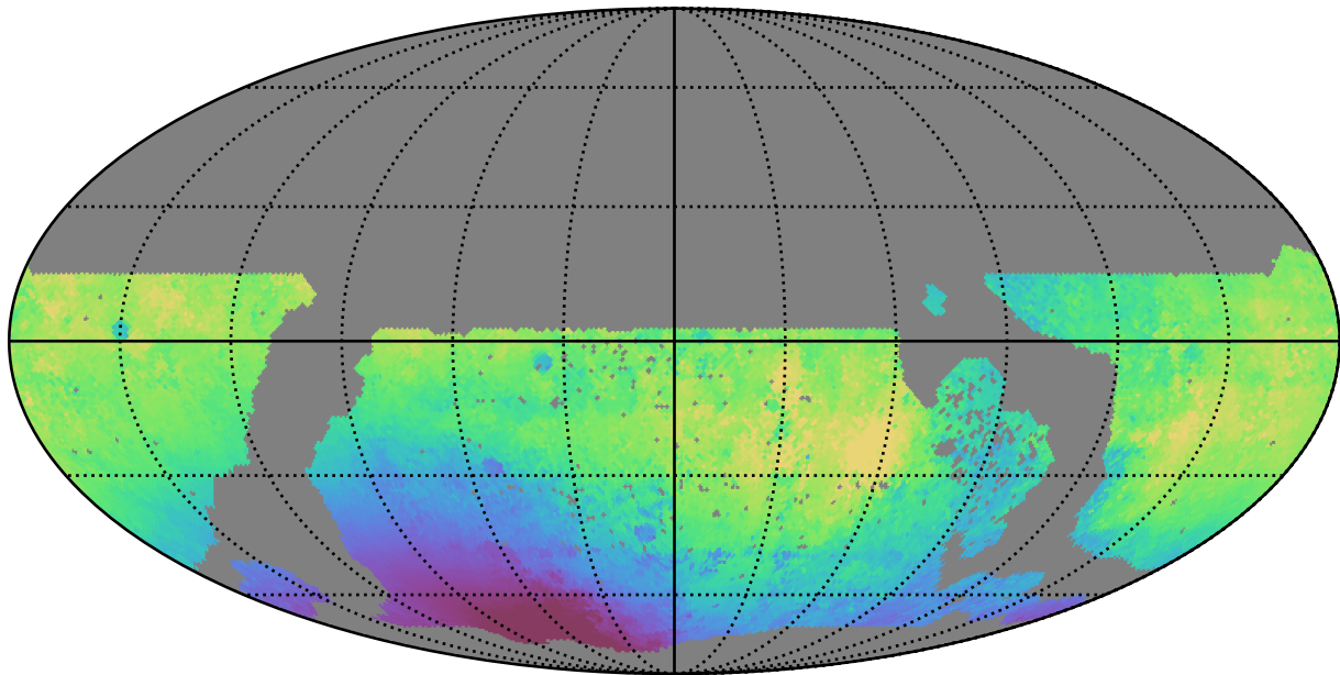
early_u_fpextra4.0_v3.4_10yrs WFD g band: Median solarElong
