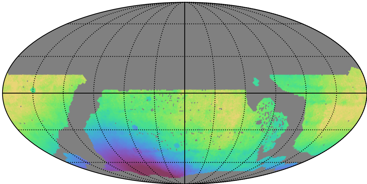
early_u_fpextra4.0_v3.4_10yrs WFD all bands: Median solarElong
