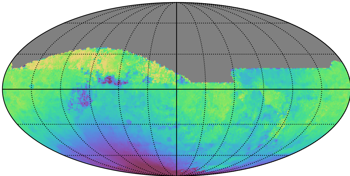
early_u_fpextra4.0_v3.4_10yrs All sky z band: Median solarElong
