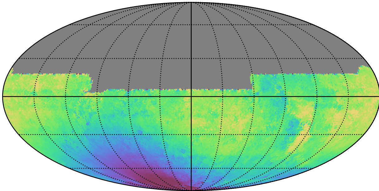
early_u_fpextra4.0_v3.4_10yrs All sky y band: Median solarElong
