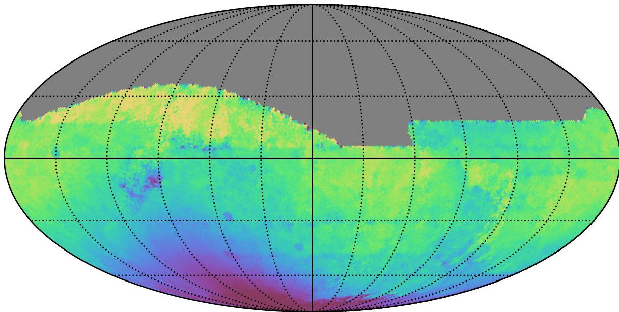
early_u_fpextra4.0_v3.4_10yrs All sky i band: Median solarElong
