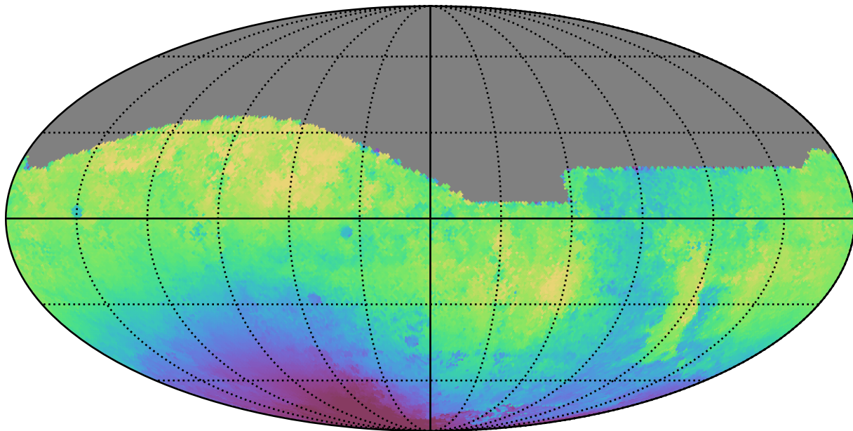
early_u_fpextra4.0_v3.4_10yrs All sky g band: Median solarElong
