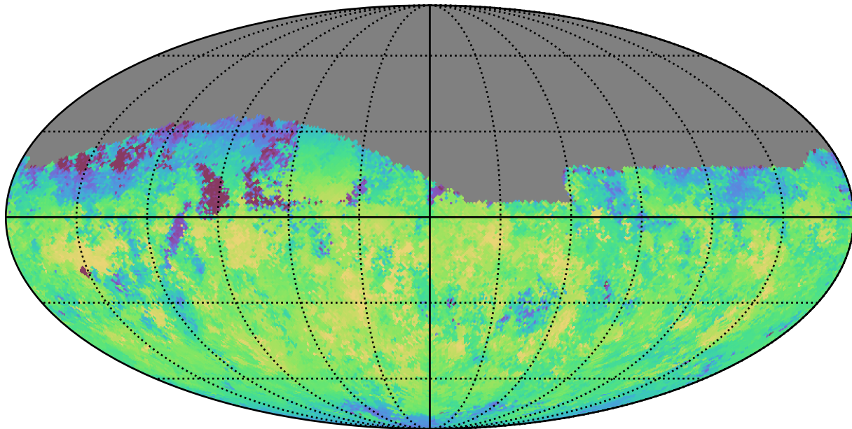
early_u_fpextra4.0_v3.4_10yrs Yr 1 z band: Median skyBrightness
