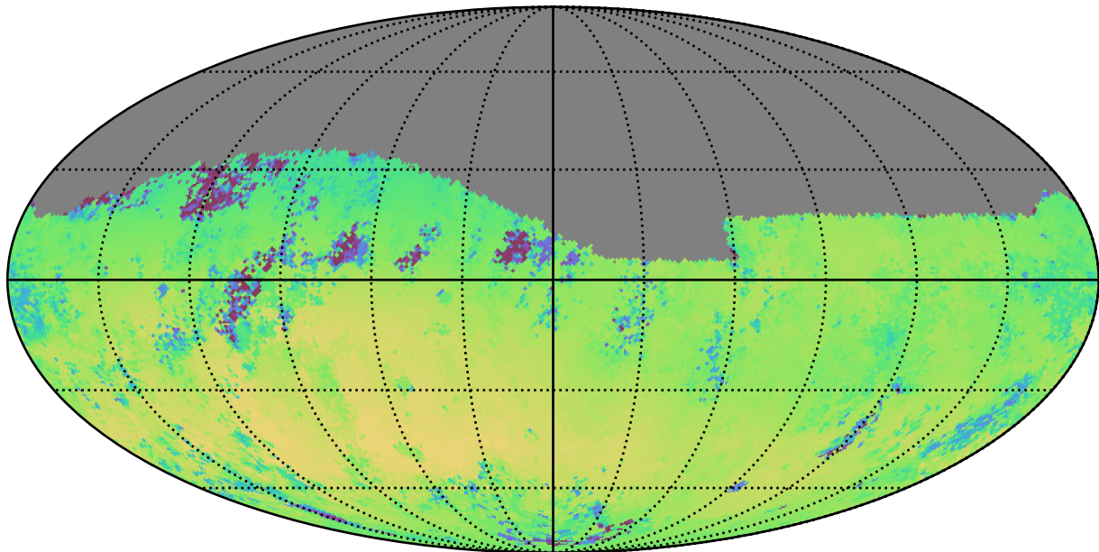
early_u_fpxtra4.0_v3.4_10yrs Yr 1 r band: Median skyBrightness
