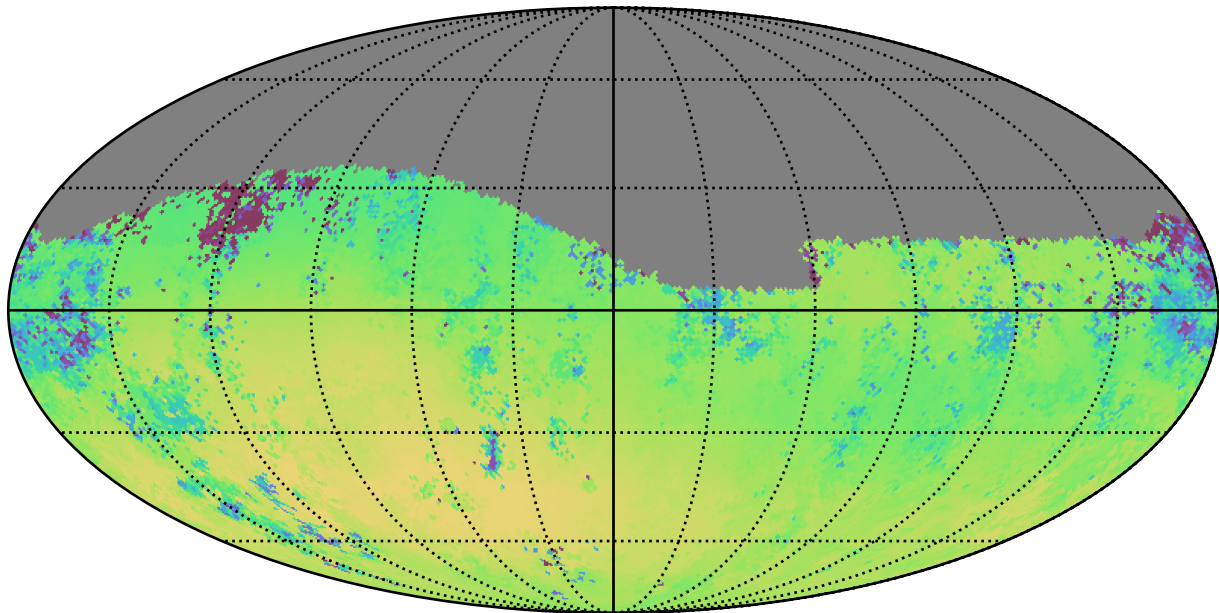
early_u_fpextra4.0_v3.4_10yrs Yr 1 g band: Median skyBrightness
