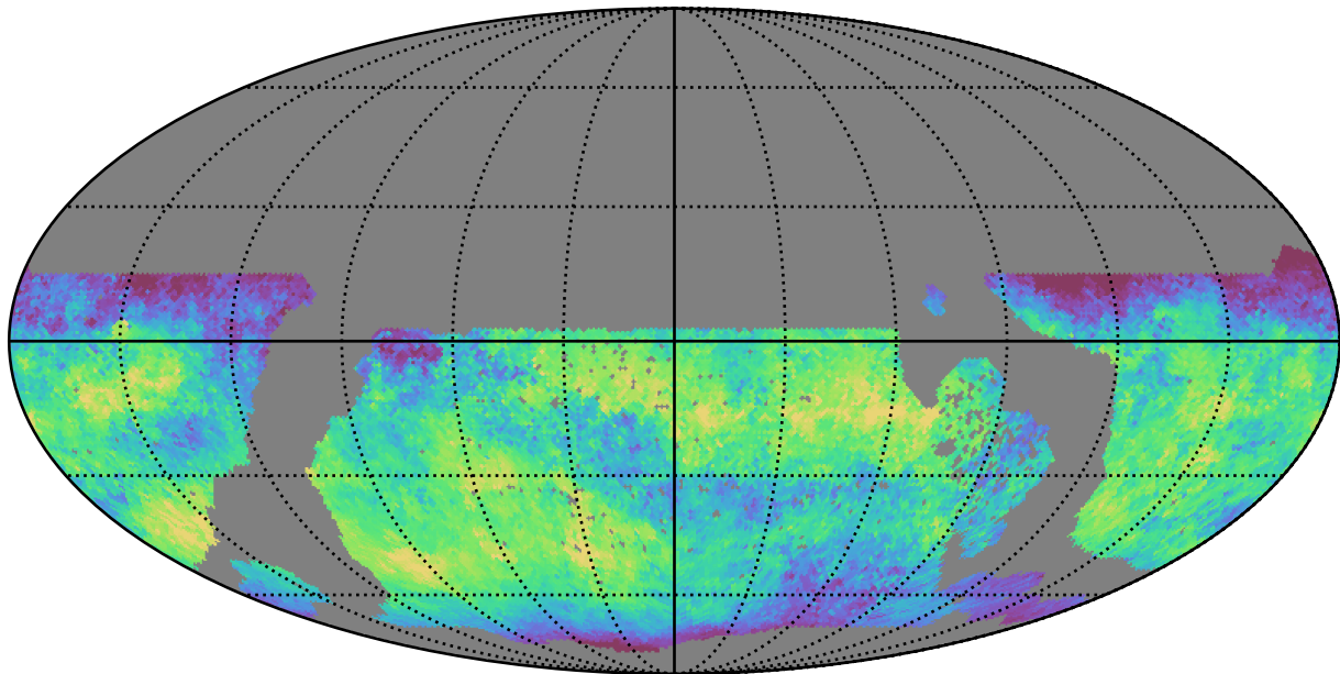
early_u_fpextra4.0_v3.4_10yrs WFD z band: Median skyBrightness
