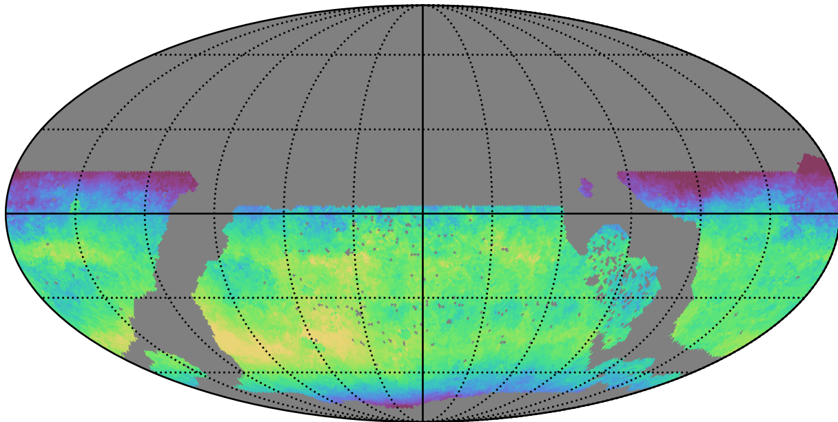
early_u_fpextra4.0_v3.4_10yrs WFD y band: Median skyBrightness
