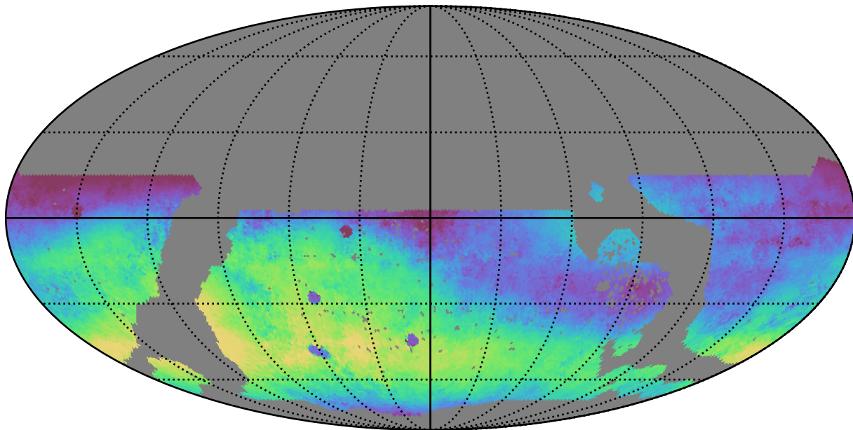
early_u_fpextra4.0_v3.4_10yrs WFD r band: Median skyBrightness
