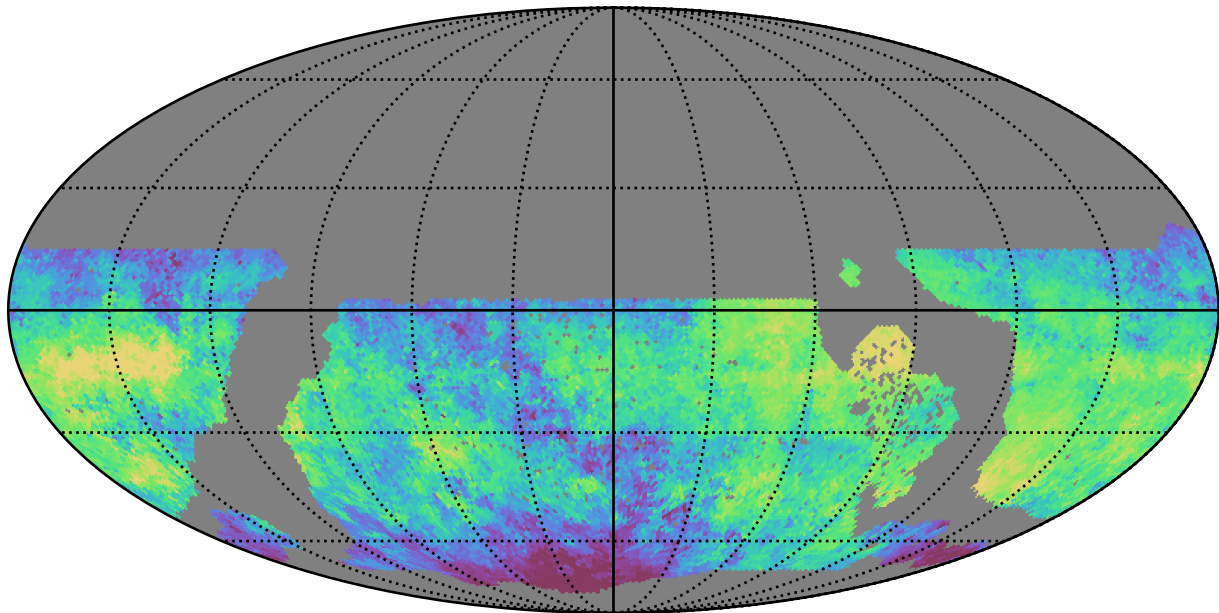
early_u_fpextra4.0_v3.4_10yrs WFD i band: Median skyBrightness
