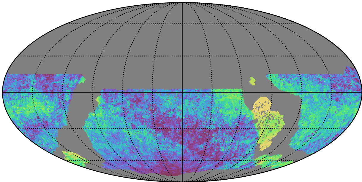
early_u_fpextra4.0_v3.4_10yrs WFD all bands: Median skyBrightness
