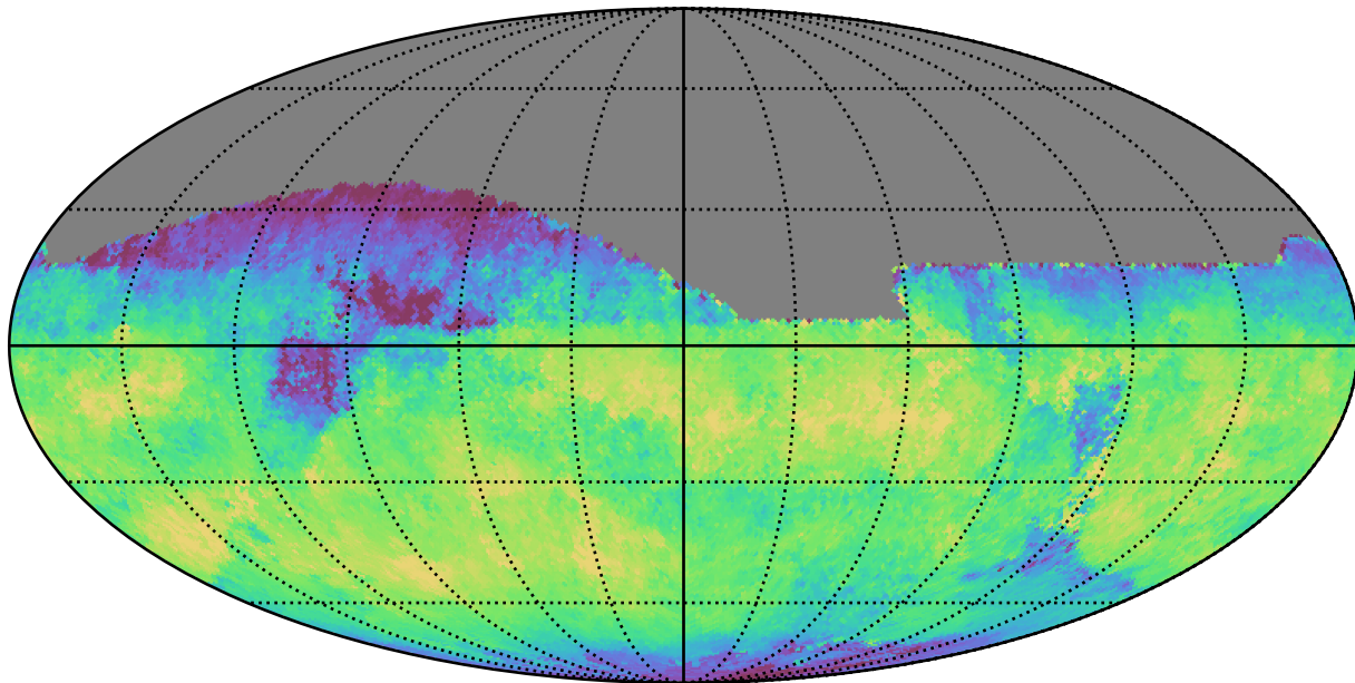
early_u_fpextra4.0_v3.4_10yrs All sky z band: Median skyBrightness
