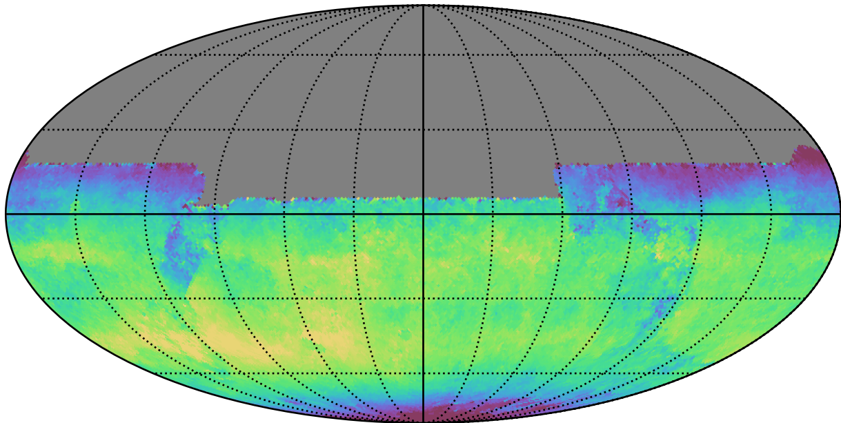
early_u_fpextra4.0_v3.4_10yrs All sky y band: Median skyBrightness
