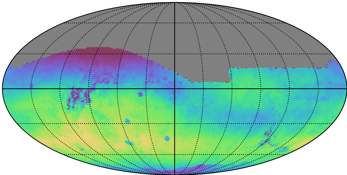
early_u_fpextra4.0_v3.4_10yrs All sky r band: Median skyBrightness
