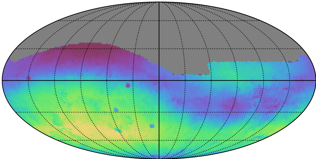
early_u_fpextra4.0_v3.4_10yrs All sky g band: Median skyBrightness
